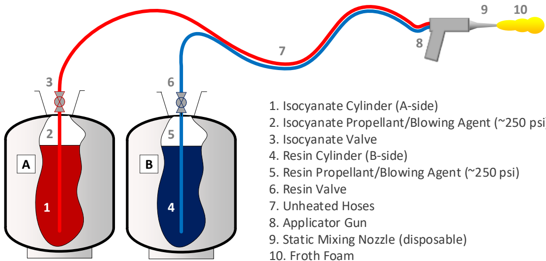
Figure 4. Schematic of a Low-Pressure SPF system
